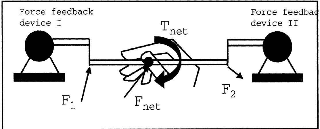
Fig. 1. Schematic of our haptic display: To display forces and torques to the user, we have connected two force feedback devices to each other through a rigid probe. This enables us to display forces in three axes and torques about two axes (the torsion about the long axis of the probe cannot be displayed with this design).
