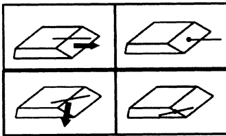
Fig. 11. Possible contact types if the projection of the probe (see appendix, Section 3) does not have a collision with the face when there is a line segment-face contact in the previous cycle: (a) point-polygon and (b) line segment-edge.
