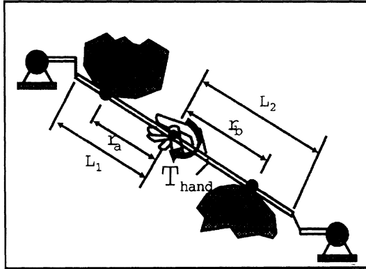
Fig. 13. Computation of interaction forces/torques when the line probe interacts with two virtual objects: The forces are distributed to the Phantoms based on the net force and moment principles.
