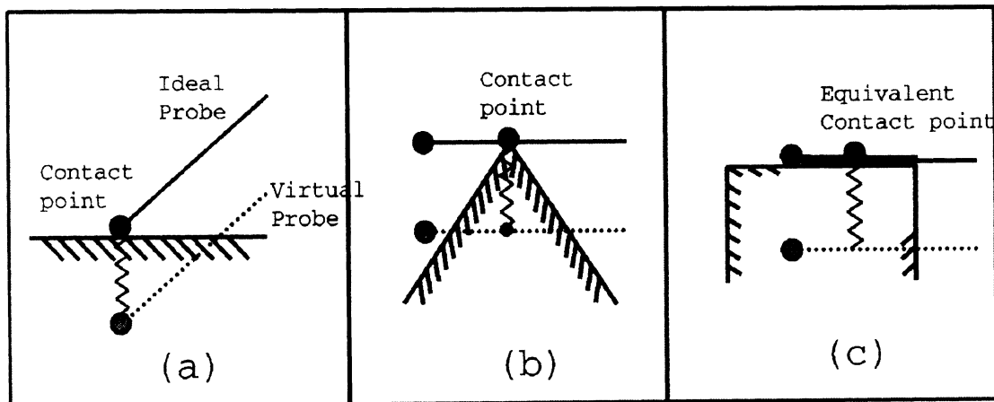
Fig. 5. Location of ideal probe relative to the virtual one for the contact conditions shown in Figure 4. Although the virtual probe can penetrate into objects, the ideal one is restricted to stay outside the objects. During the interactions, the collisions of the virtual probe with objects are detected and the collision information is used to calculate the location of the ideal probe. The stretch of the spring between the ideal and virtual probes in the figure illustrates a method for computing force interactions between the probe and the convex object for three different contact conditions.
