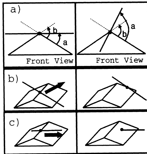
Fig. 8. Possible collision situations following a line segment-edge contact.
