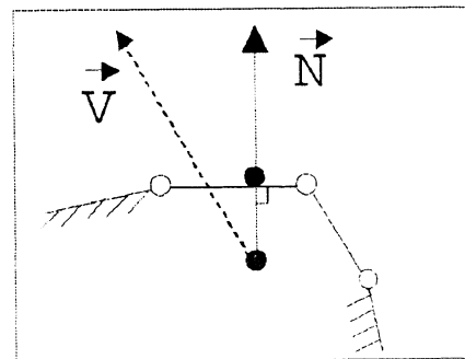
Fig. 6. A point-polygon collision: In this figure, one end of the probe is already inside the object whereas the other end point is outside the object.
