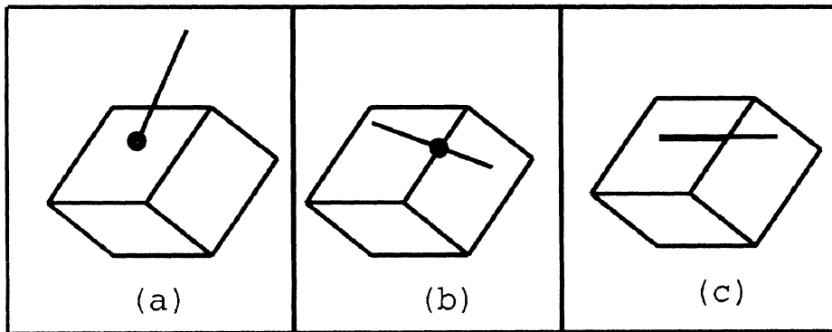
Fig. 4. Possible contact conditions for the line segment-convex object interactions: (a) the probe contacts a polygon of the object at a single point (point-polygon), (b) the probe intersects an edge of the convex object at a single point (line segment-edge), (c) the probe stays on the surface of a plane constructed from a single or multiple polygons, and the intersection between the probe and the plane is either a portion or all of the probe (line segment-face).
