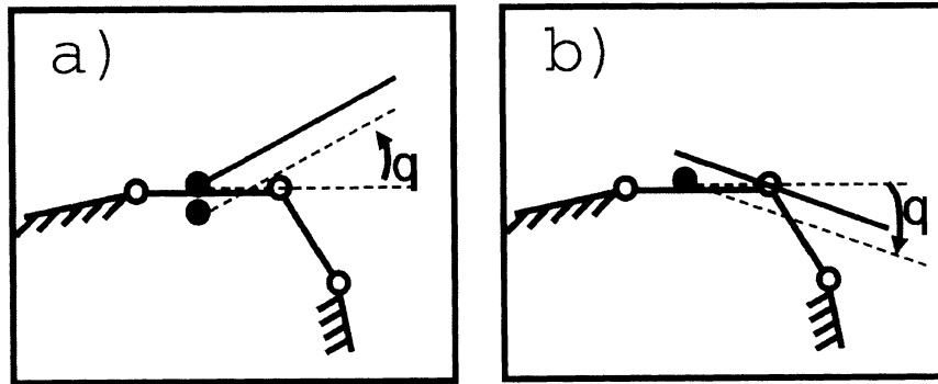
Fig. 10. Possible future contacts if \theta becomes larger than epsilon and the projection of the line probe has a collision with the face in line segment-face contact: (a) point-polygon, (b) line segment-edge.
