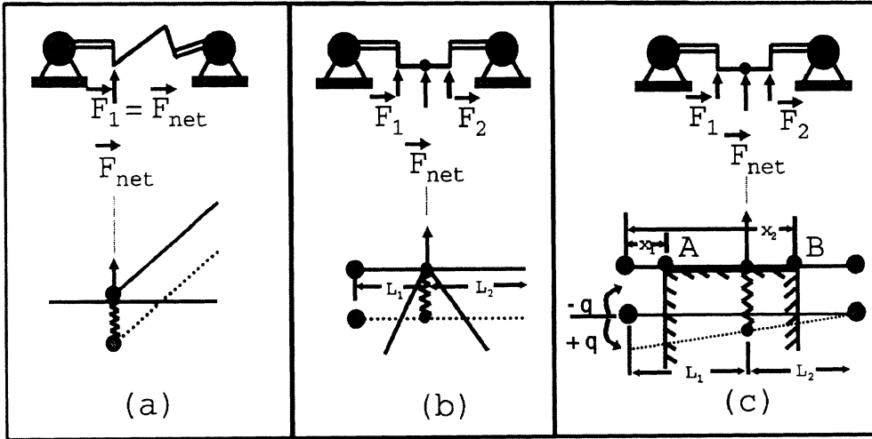
Fig. 12. The collision response for ray-based haptic rendering: The ideal location of the probe is determined based on the type of collision (i.e., point-polygon, line segment-edge, or line segment-face). In the figure, dashed and solid lines represent the virtual and ideal probes, respectively.
