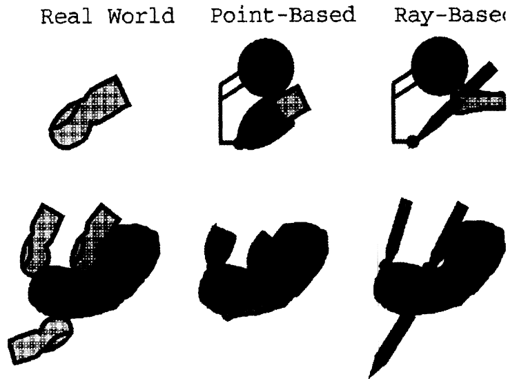
Fig. 2. The difference in point- and ray-based rendering techniques: In point-based rendering, the haptic probe is modeled as a single point leading to artifacts such as feeling the bottom surface of the object by passing through the object. In ray-based rendering, collisions between virtual objects and end-points as well as side of a line segment are detected.
